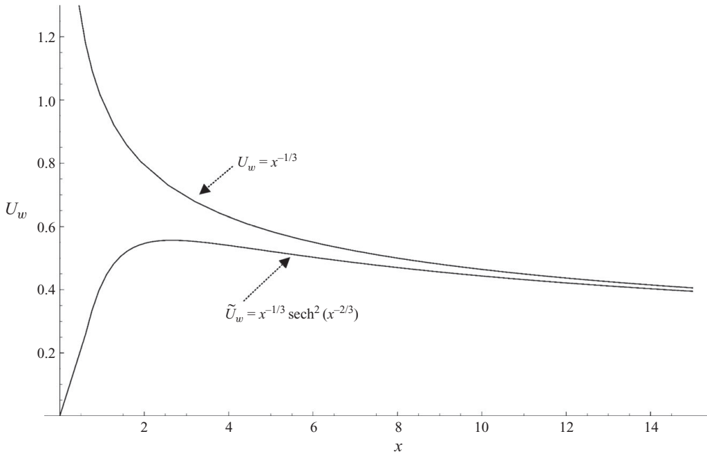
FIGURE 1. Shapes of the stretching velocity distributions U_w and \tilde{U}_w corresponding to the Bickley solution (7.1) and its transformed counterpart (7.14) obtained by a constant translation y_0 of the transverse coordinate y (the velocities have been expressed in units of (6a^3\nu/y_0^2)^{1/4} and the coordinate x in units of (ay_0^2/6\nu)^{3/4} ).
